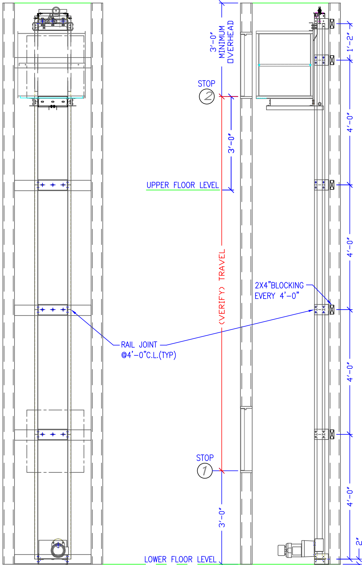
B-B DUMBWAITER SHAFT
