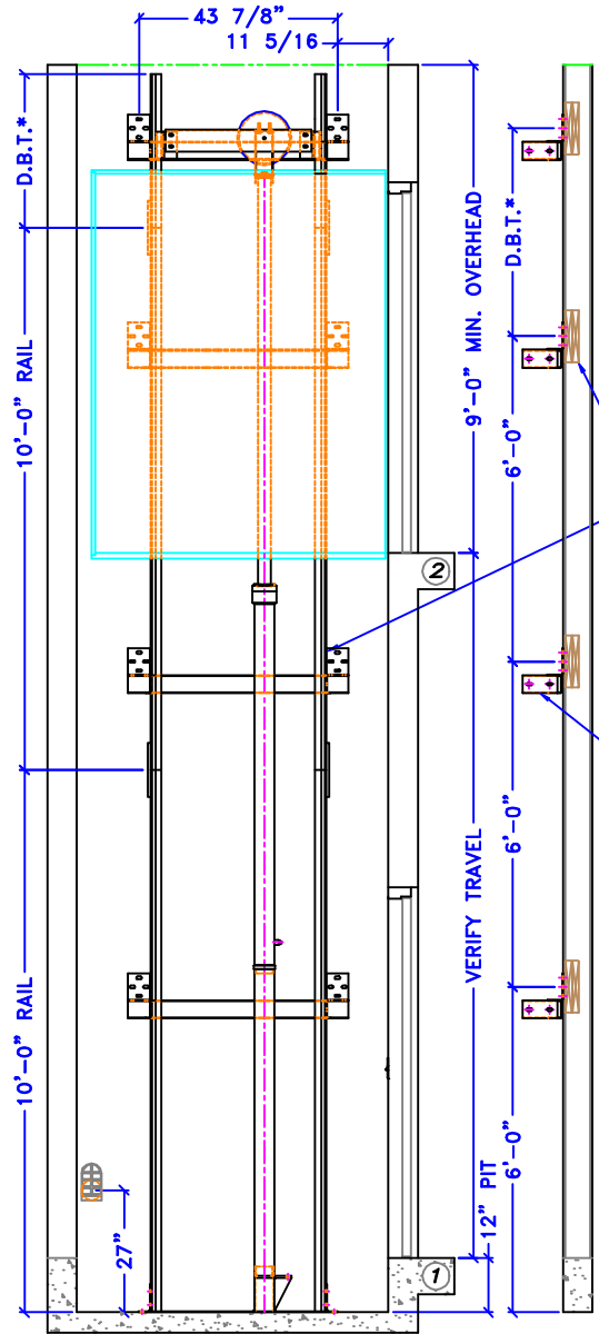
C-C HOISTWAY ELEVATION (A-A) BRACKET LOCATIONS *DETERMINED BY TRAVEL
