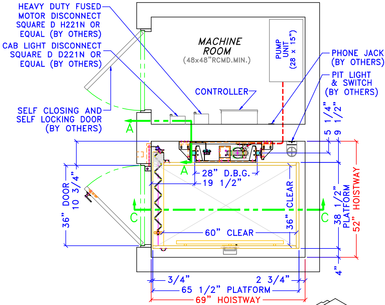
HOISTWAY PLAN
